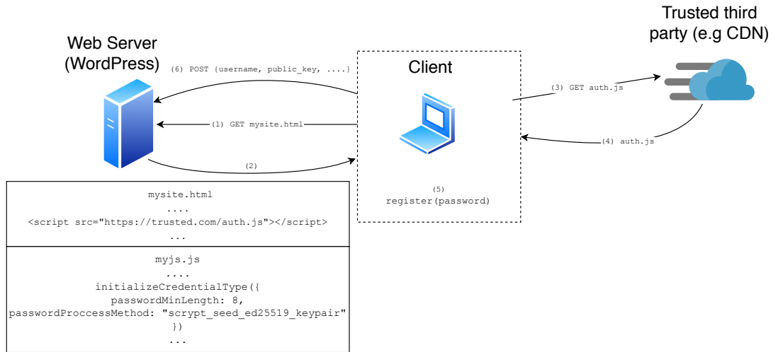
Fig. 1. Overview of the architecture of auth.js . The client requests the web application from the server (1). The server responds by sending the html file, which directs the client to retrieve auth.js from a trusted third party, as well as with a JavaScript file in which the authentication options are initialized (2). The client then retrieves auth.js from the trusted source (3 and 4). The client's browser prompts the user for a password and the register API call from auth.js is used to generate the correct credential (5). In this case the generated credential is the user's public key, which is generated based on the password which the user provided. Finally, the credential is sent to the server (6), where it will be verified.
